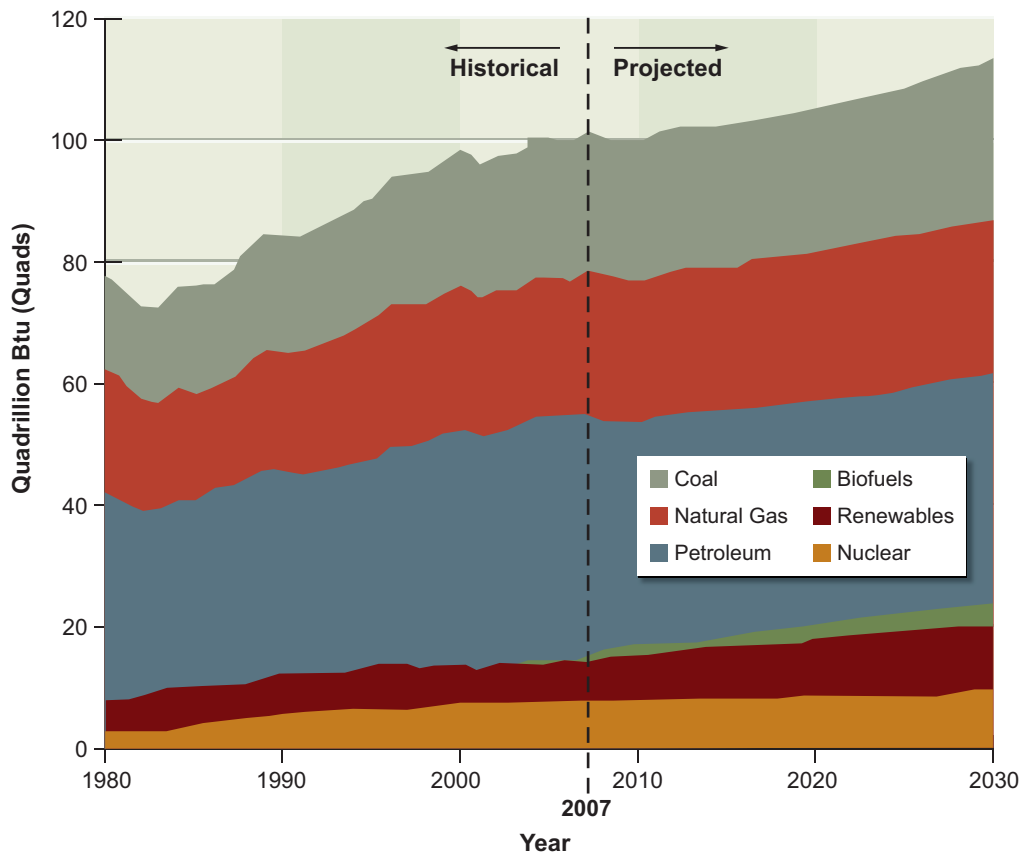
FIGURE 1.7 Historical (1980–2007) and projected (2008–2030) energy consumption in the United States by primary energy source, in quads. The projected energy use from 2020 to 2030 reflects the U.S. Energy Information Administration’s (EIA’s) 2008 reference case; this reference case assumes that current policies that affect energy supply and consumption will remain unchanged and that economic growth rates and technology development and deployment trends will continue over the next 20 years. As explained in Box 2.1 in Chapter 2 and in Annex 3.A in Chapter 3, the AEF Committee uses the EIA reference case as the reference scenario for its study. Source: Energy Information Administration, 2008b.
